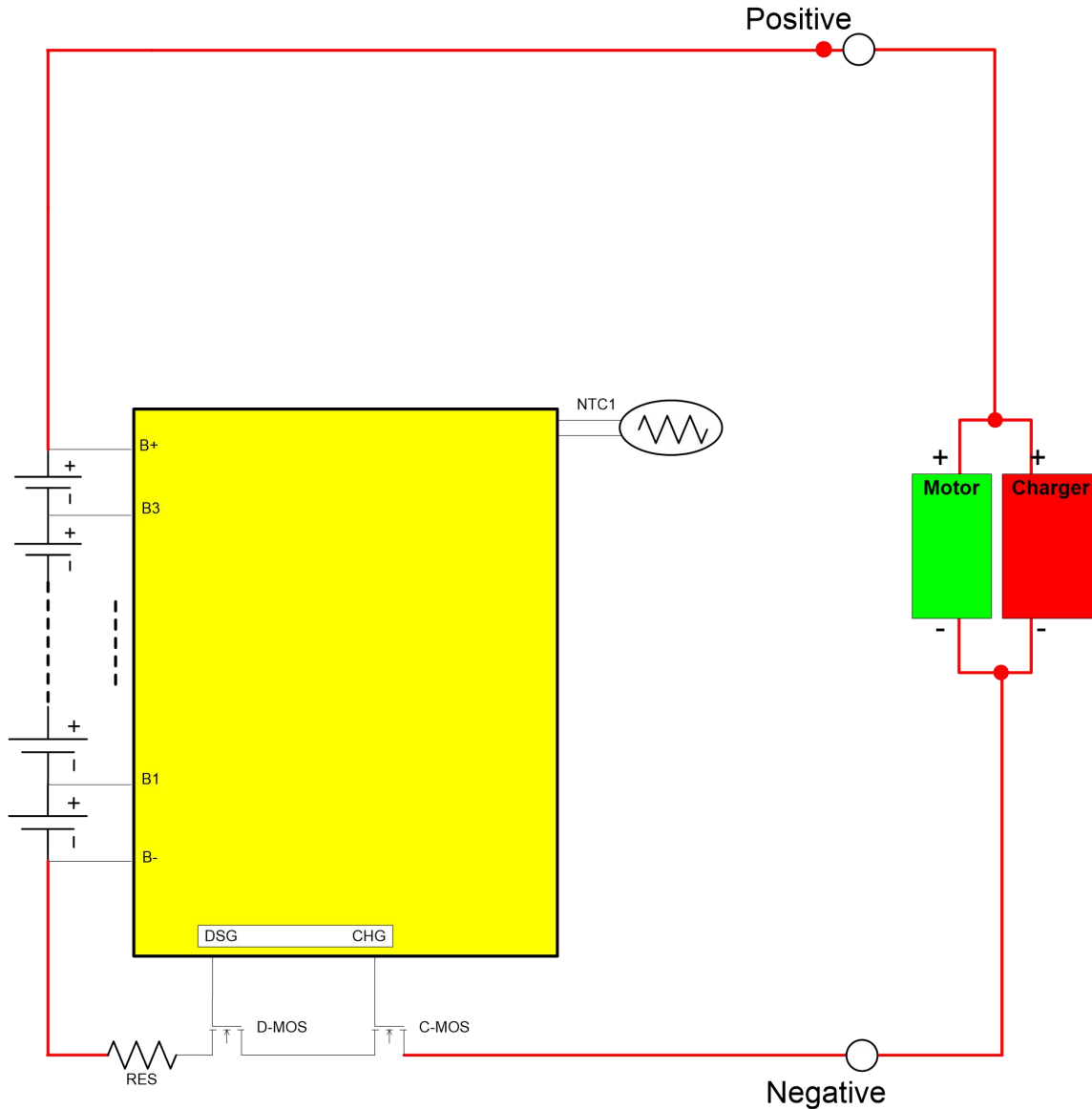
Figure 1. Schematic Diagram of Battery System
